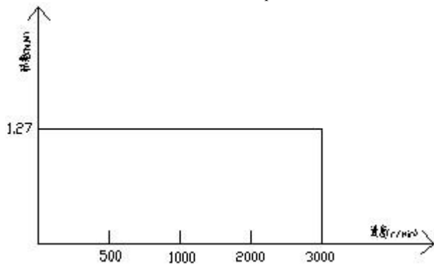
iHSV60-30-20-36-XXX4/5000 Torque characteristics
